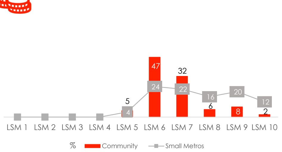
LSM distribution
